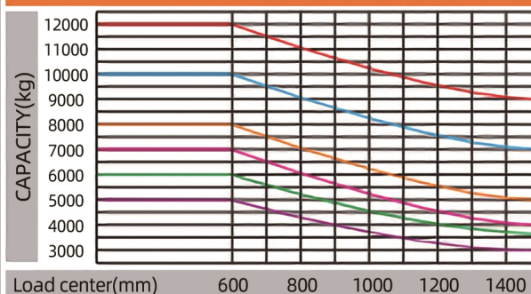
Load curve
